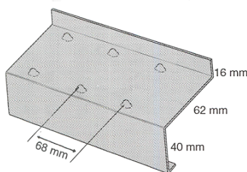
KADERPROFIEL BR 40/62 Aluminium
